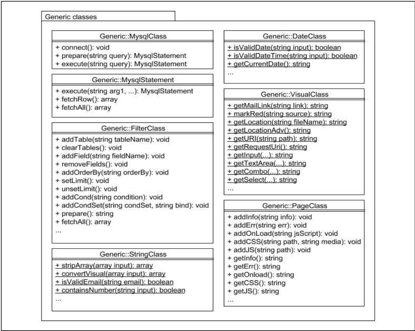
Figure 1.3.2. Class diagram for generic classes
